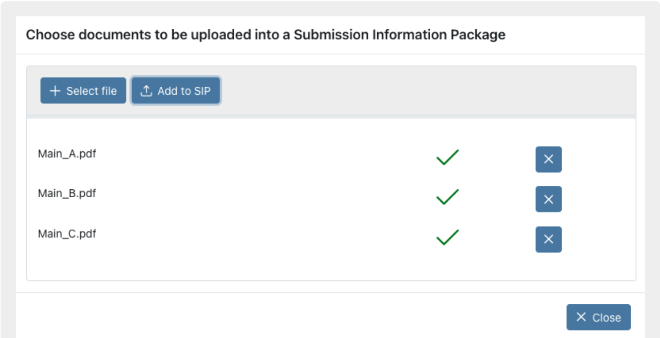
Figure 23. File upload.
